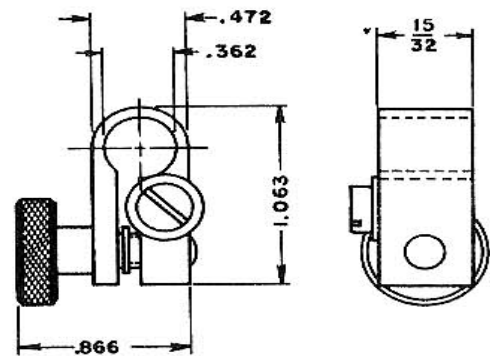
FILAMENT CONNECTOR S-3707
