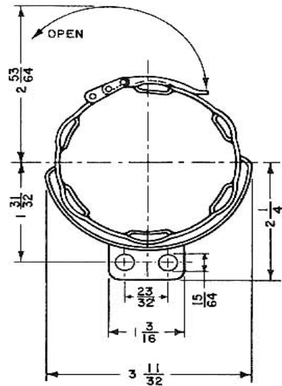
GRID CONNECTOR S-17288
