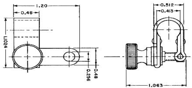
FILAMENT CENTER PIN CONNECTOR S-21000
