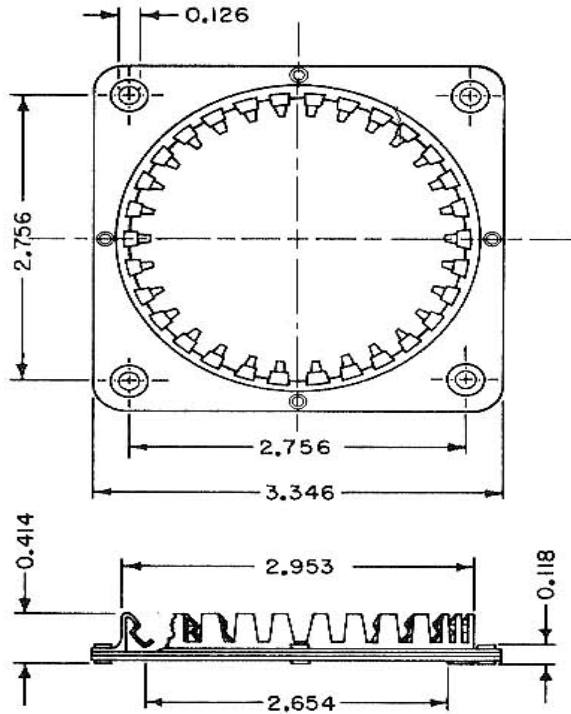
GRID CONNECTOR S-3706
