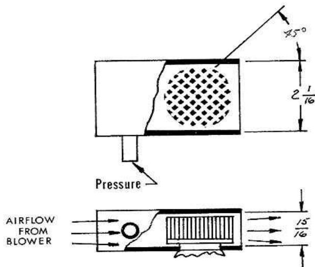
- COWLING DETAIL -
