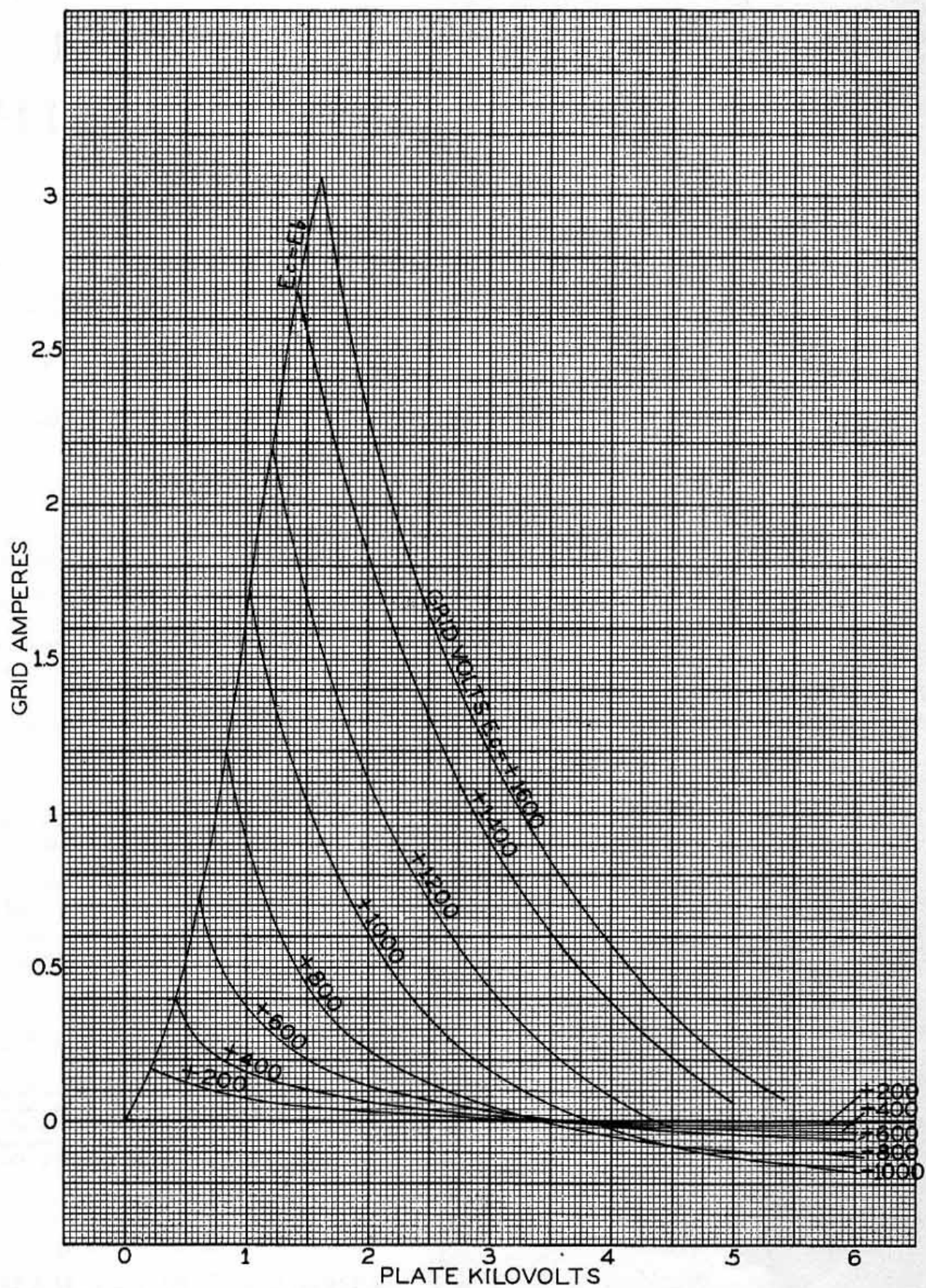
AVERAGE GRID CHARACTERISTICS F-101-B Transmitting Tube
