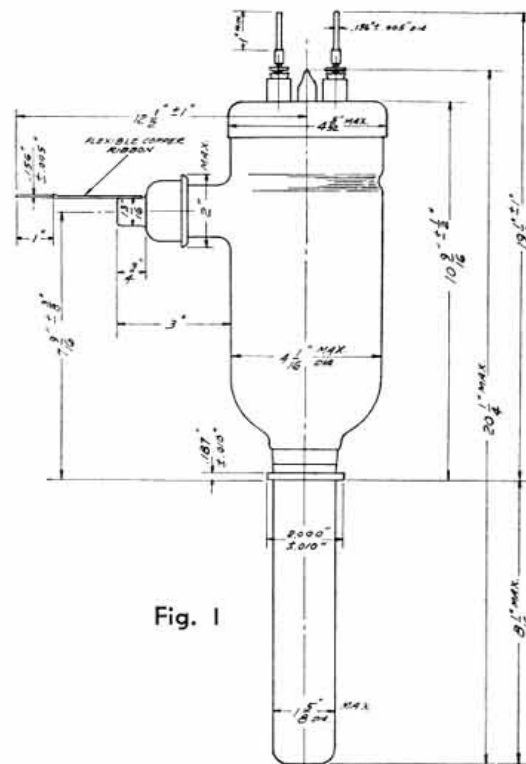
Outline Drawing
