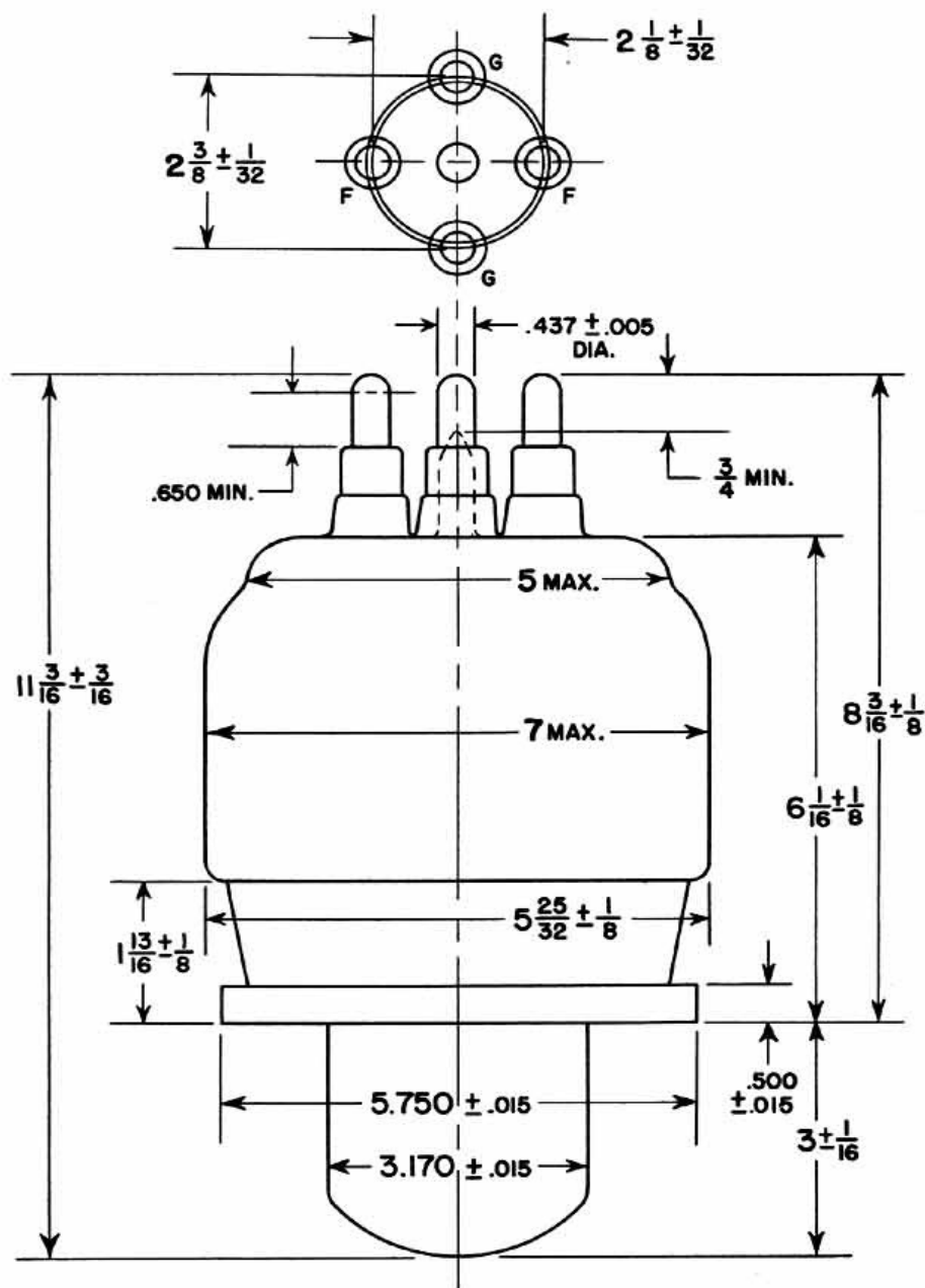
OUTLINE DRAWING F-5658
