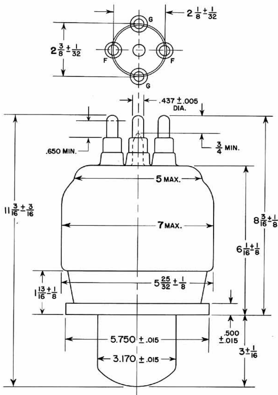
OUTLINE DRAWING F - 5771
