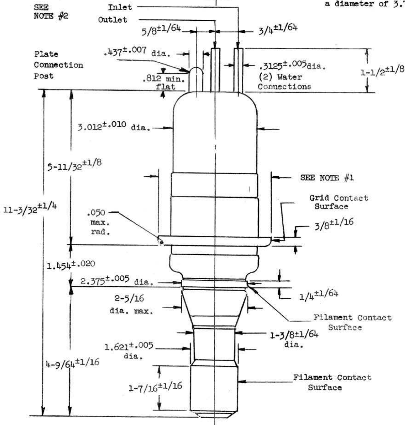
OUTLINE F-6401 PULSE TRIODE
