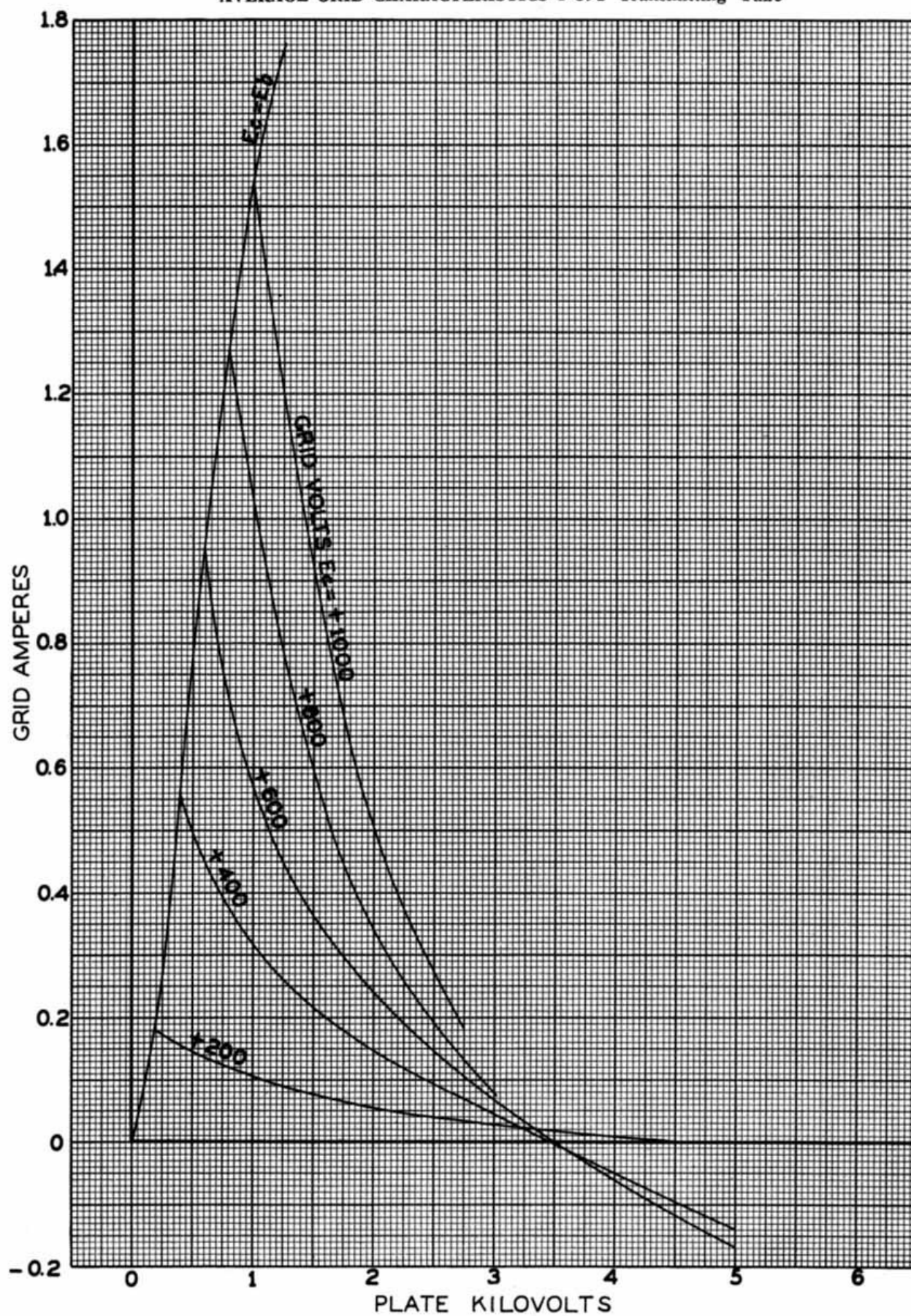
AVERAGE GRID CHARACTERISTICS F-891 Transmitting Tube
